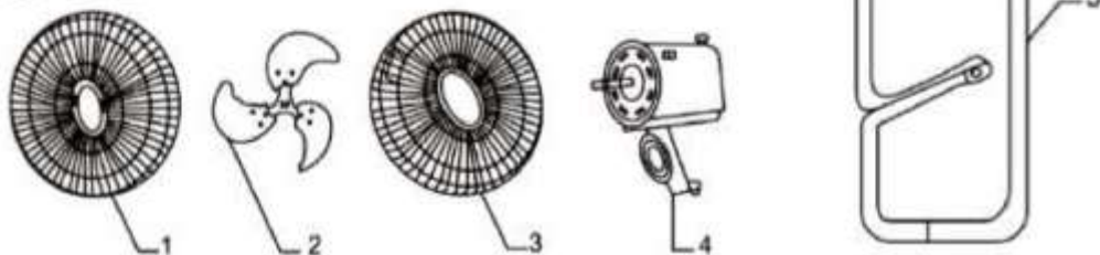
1. Front Guard; 2. Blades; 3. Back Guard; 4. Motor; 5. Foot stand
